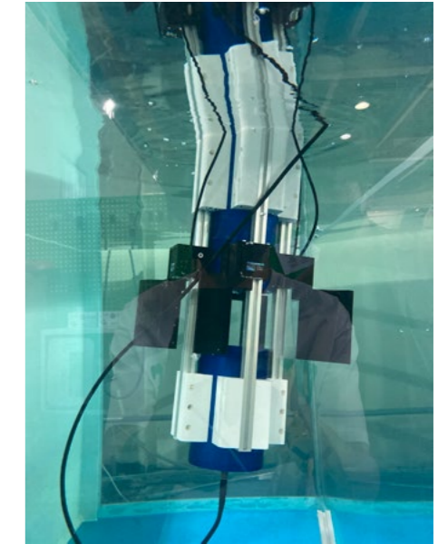
▲ Hardware Testing of the Underwater Microscope in a Water Tank (Nov 2022)
